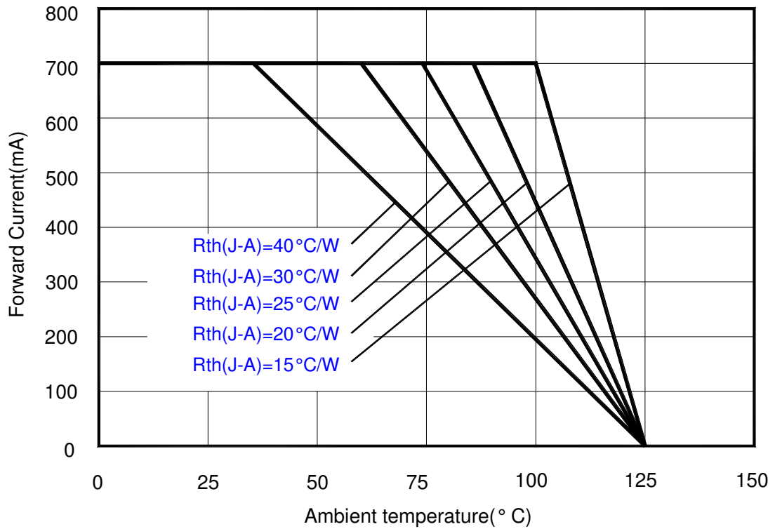
<Figure 10 Forward current & ambient temperature at 700mA>
