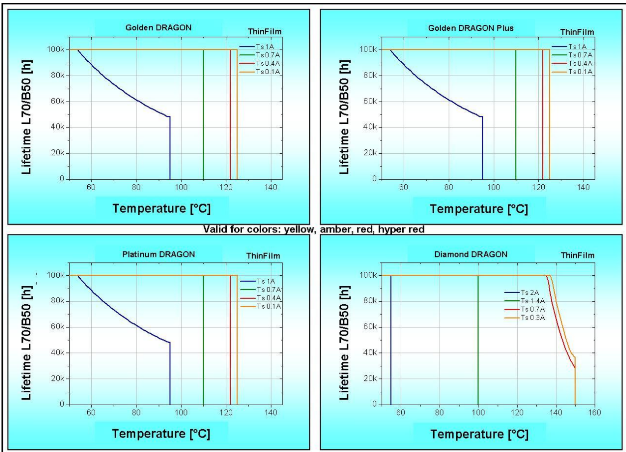
Figure 7: Lifetimes (*) of various DRAGON LED with ThinFilm technology with respect to T_s
